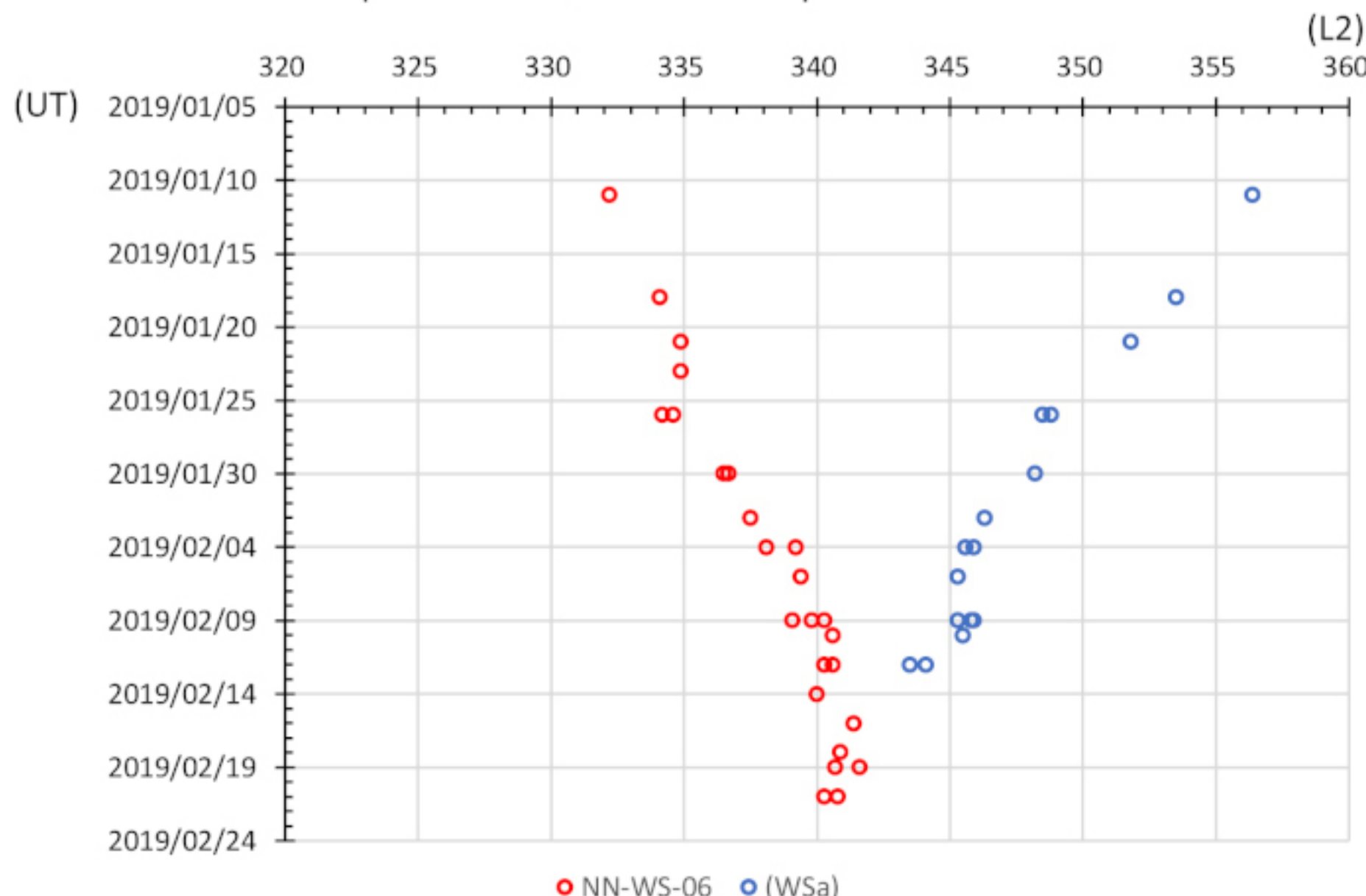
Jupiter in 2019 / N2 White Spots Drift Chart
