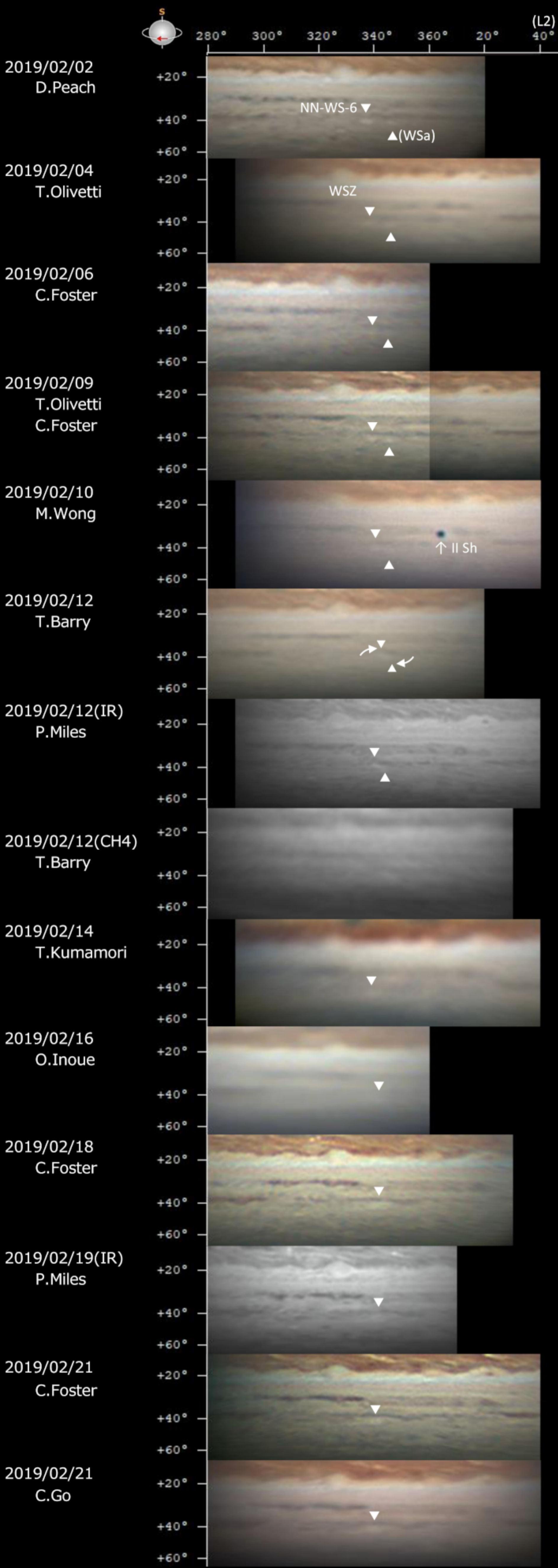
Jupiter in 2019 / N2 White Spots Drift Chart
