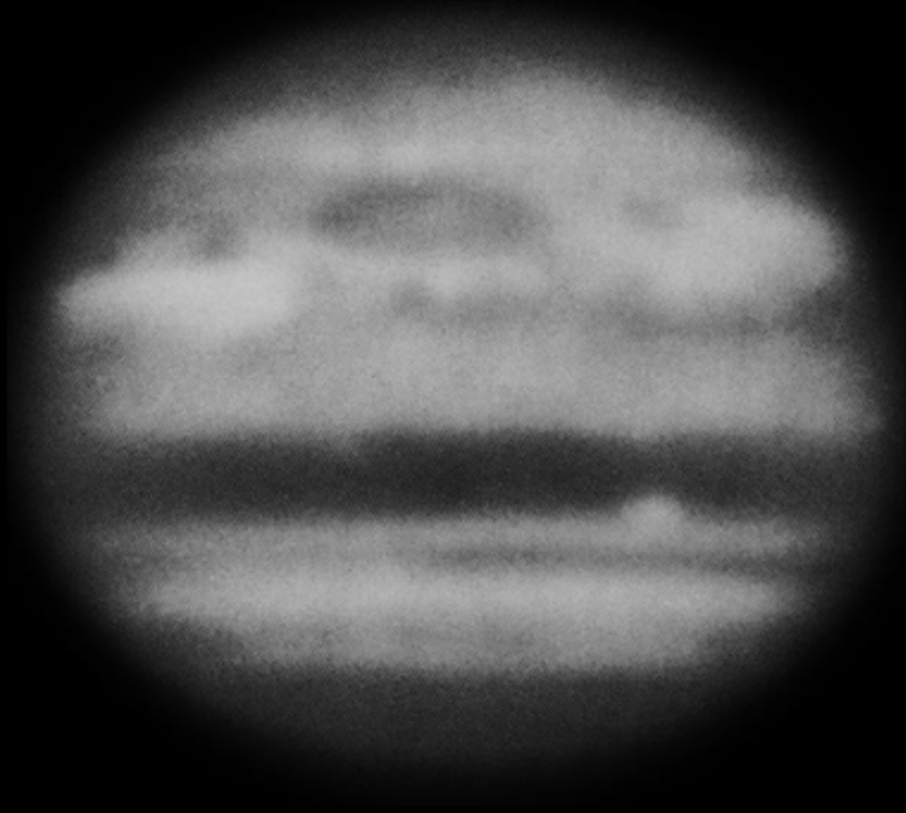
1928-10-07 (B) Lowell
