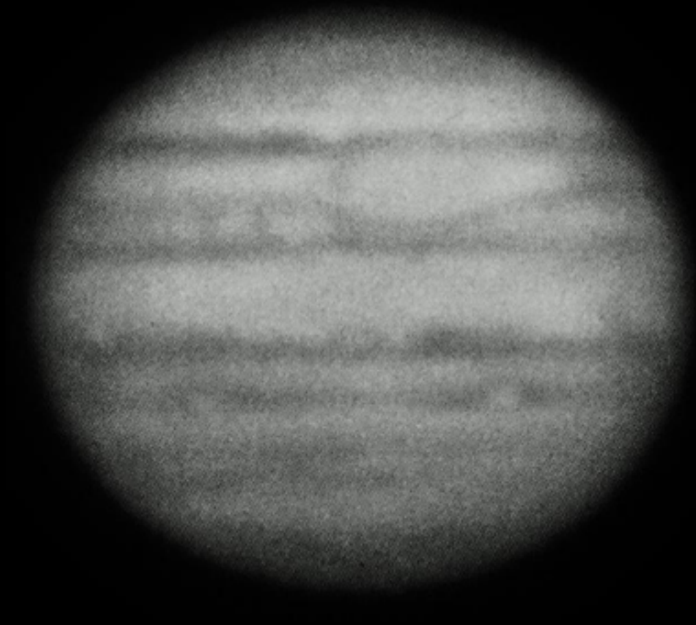
1914-09-03 (Y) Lowell
