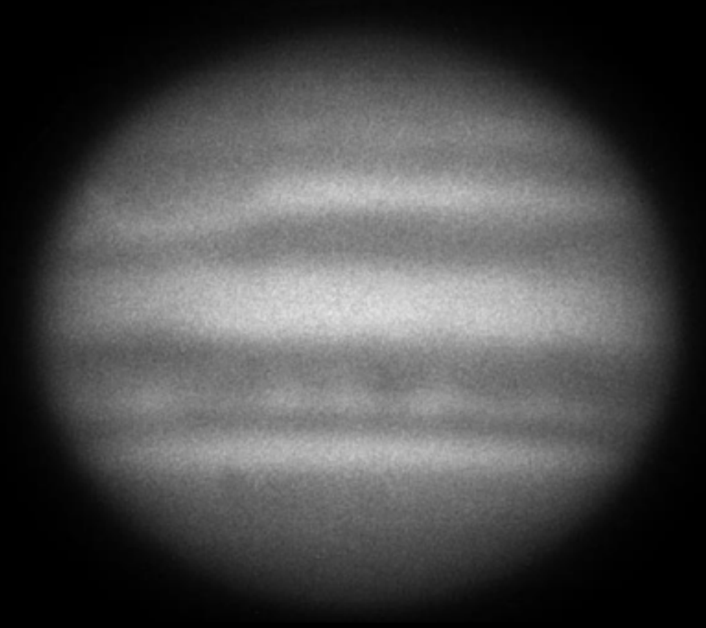
1893-11-15 (Y) Lick
