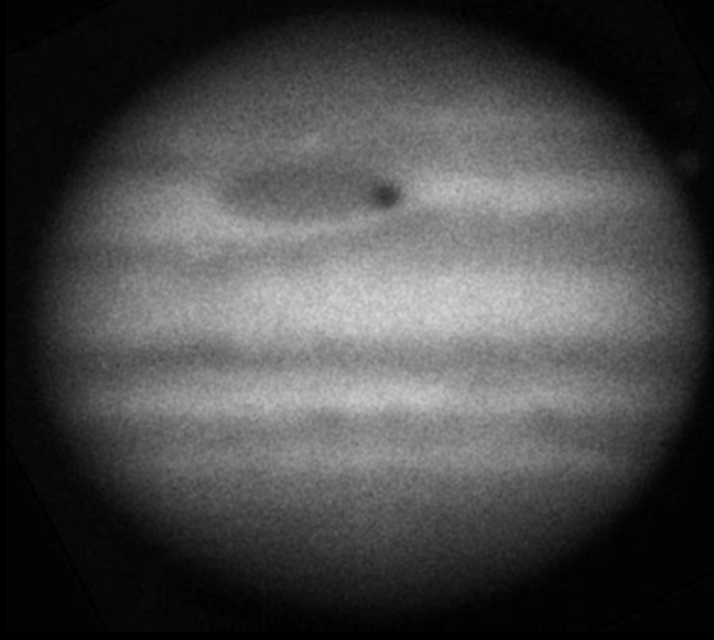
1891-08-20 (Y) Lick
