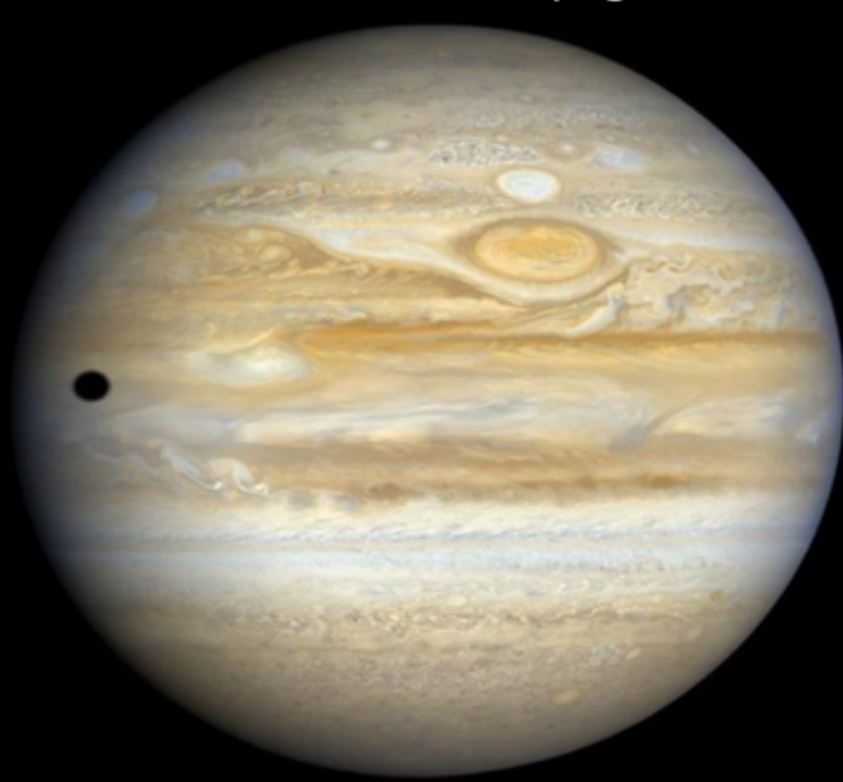
1979-07-08 Voyage 2
