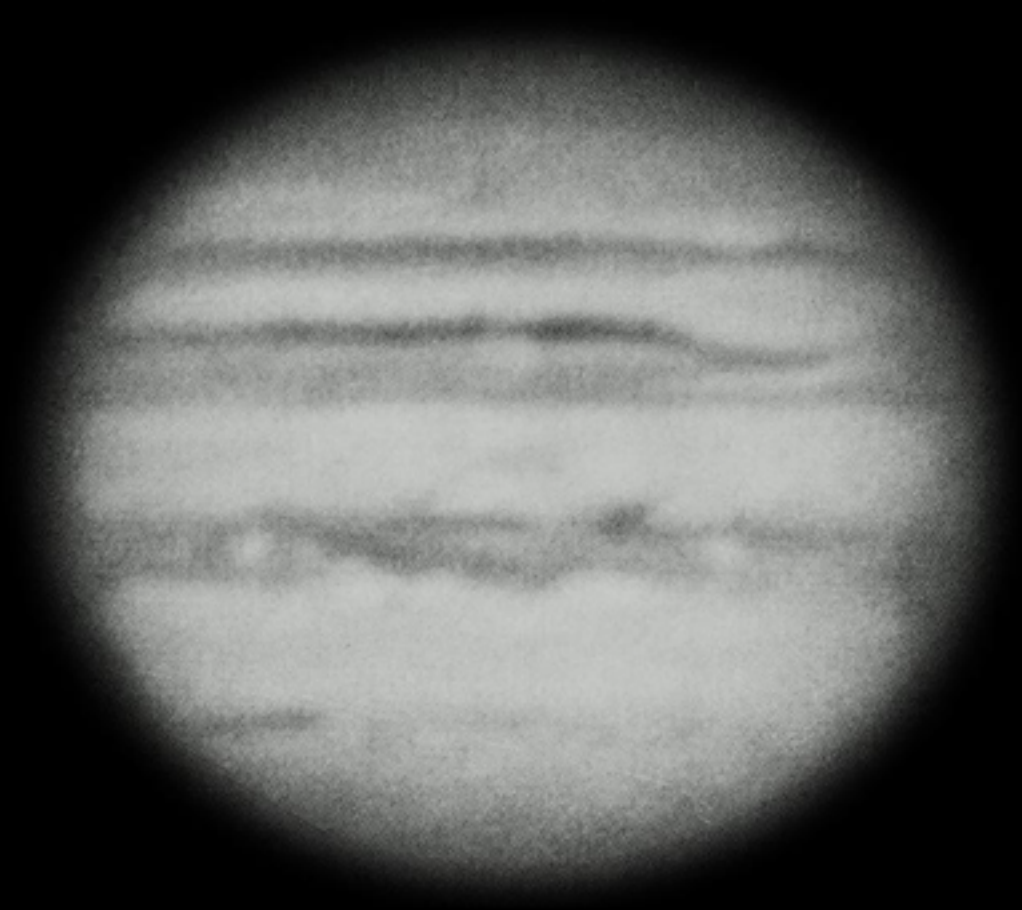
1915-10-20 (Y) Lowell
