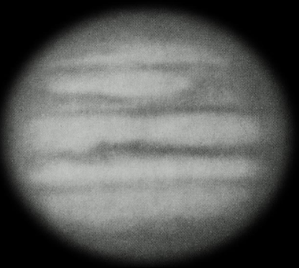
1917-12-20 (Y) Lowell
