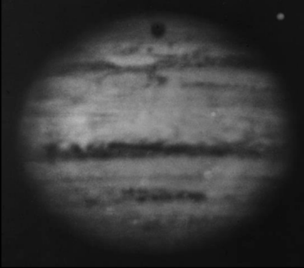
1952-10-23 Mt. Palomar
