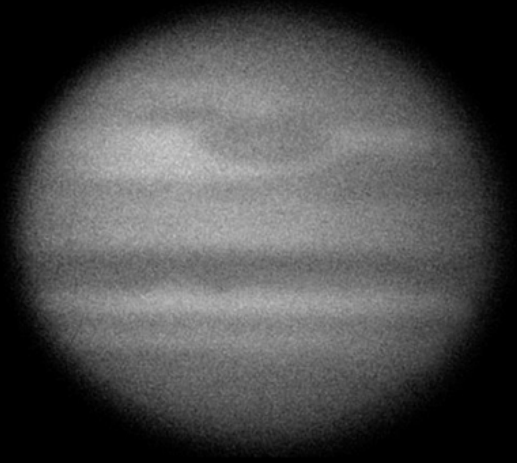
1890-09-22 (Y) Lick
