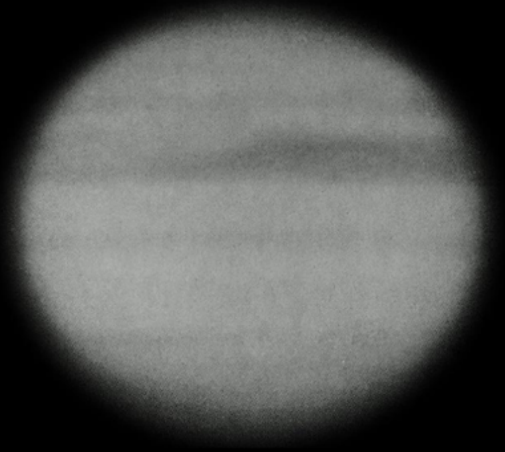
1904-10-28 (Y) Lowell
