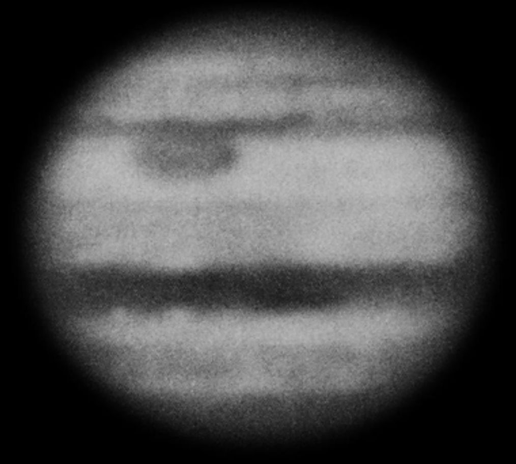
1936-07-05 (Y) Lowell
