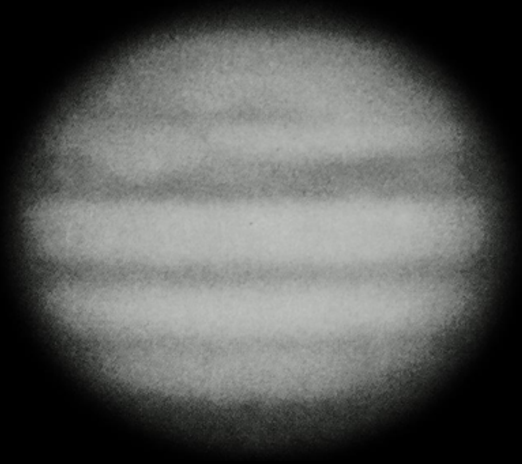
1911-05-06 (Y) Lowell
