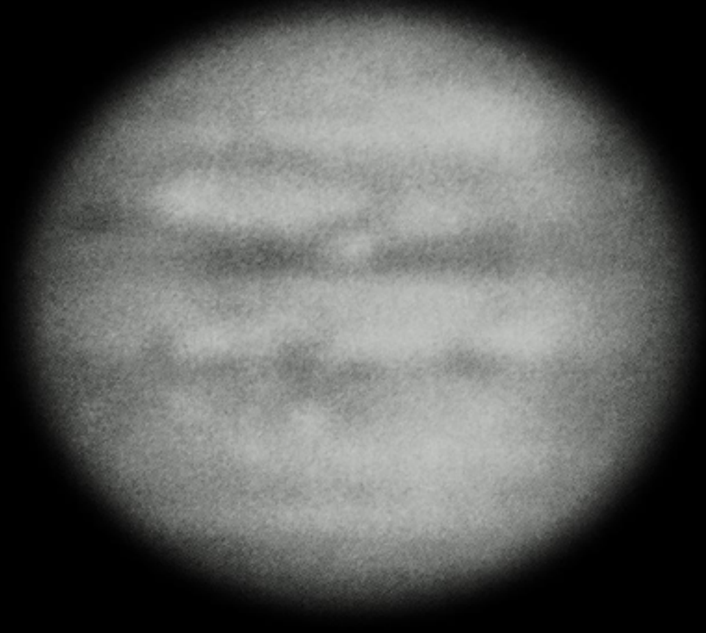
1913-08-17 (Y) Lowell
