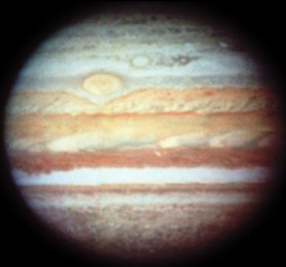
1991-10-11 HST
