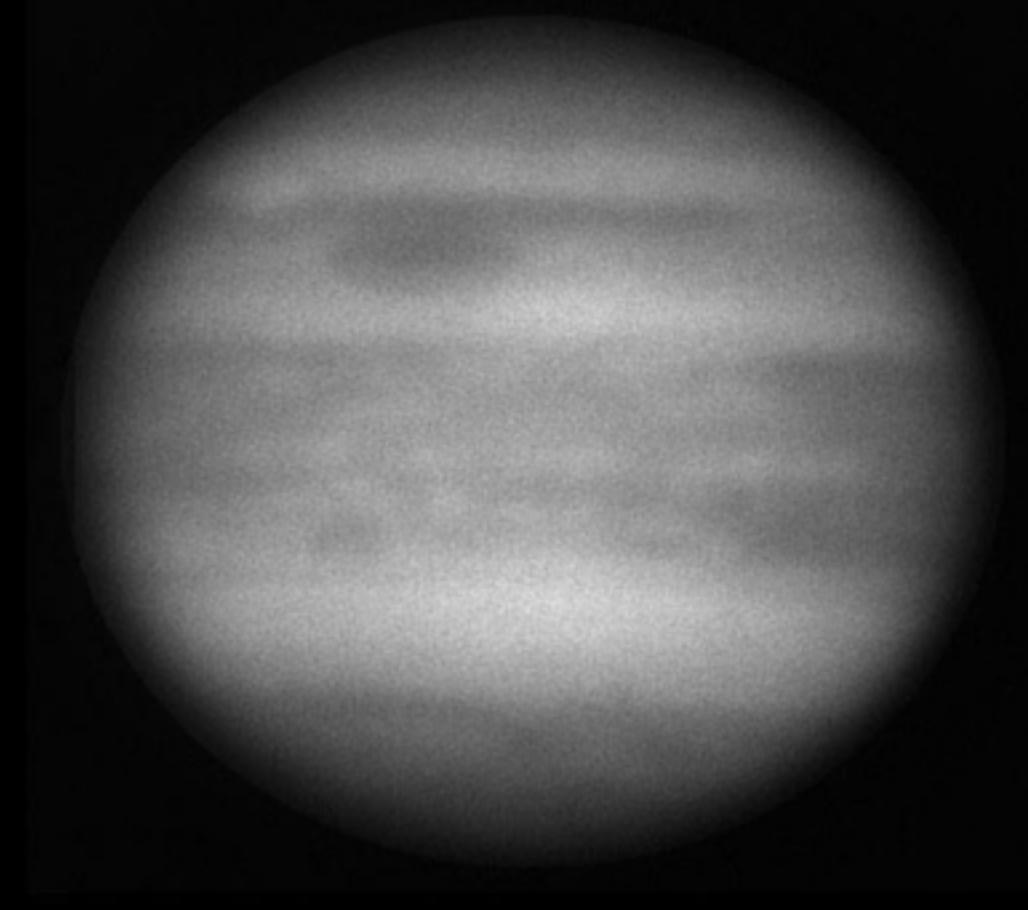
1963-09-08 Saint-Michel
