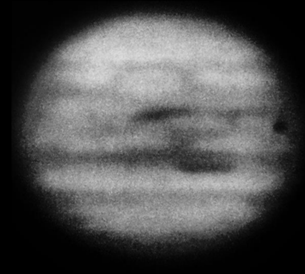
1938-08-11 (Y) Lowell
