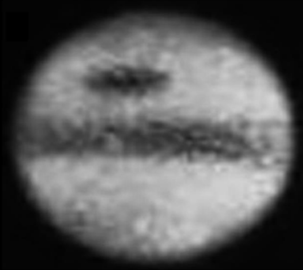
1879-09-03 A.A. Common
