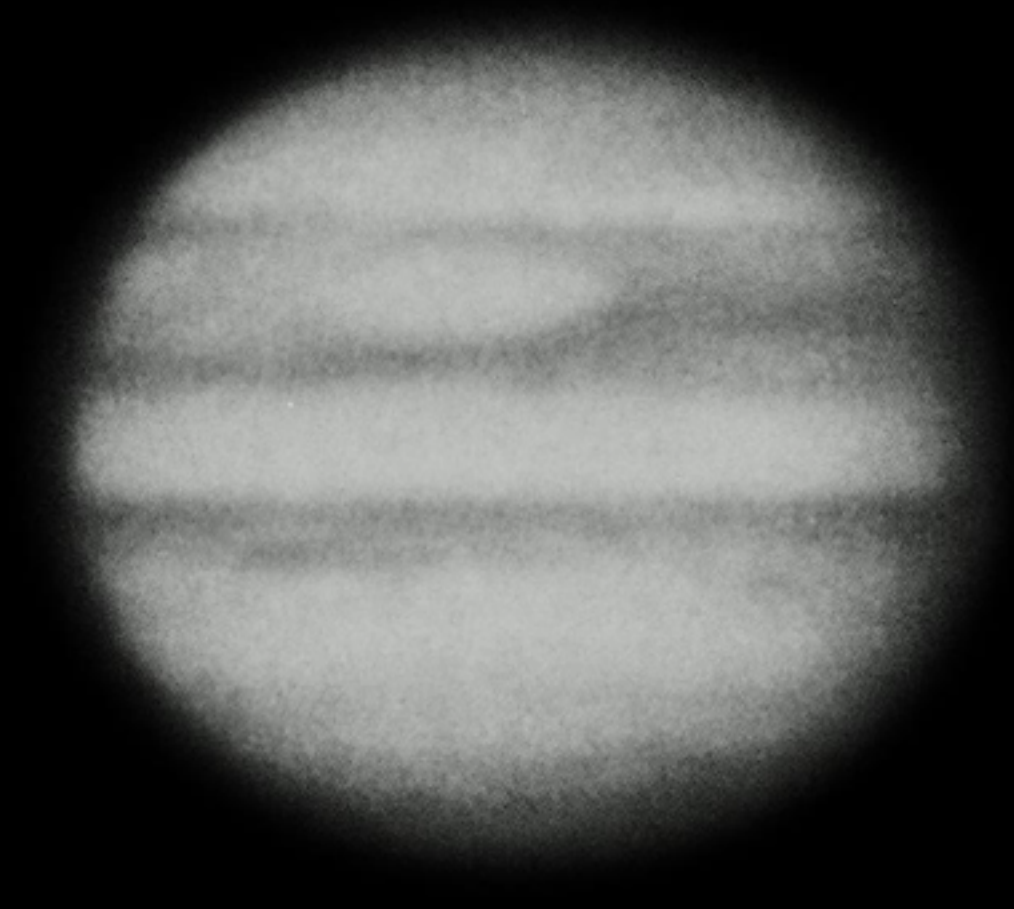
1908-08-16 (Y) Lowell
