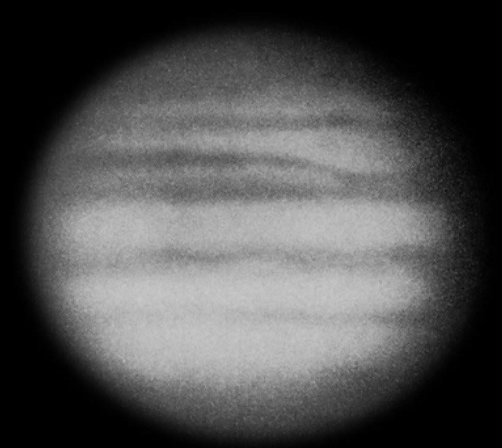
1931-02-28 (Y) Lowell
